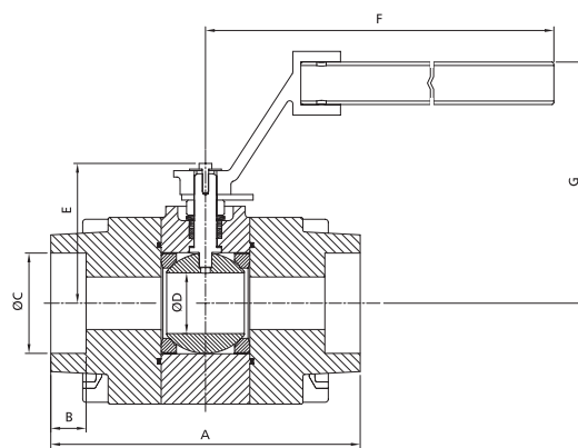
Socket-weld end
