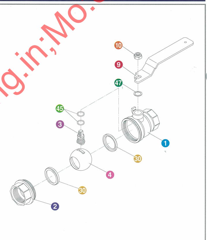
* Illustration shows threaded ends design up to 2".
